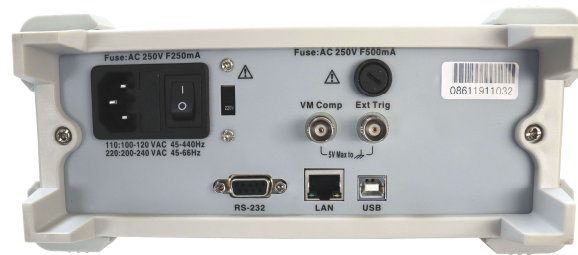
Rear Panel
